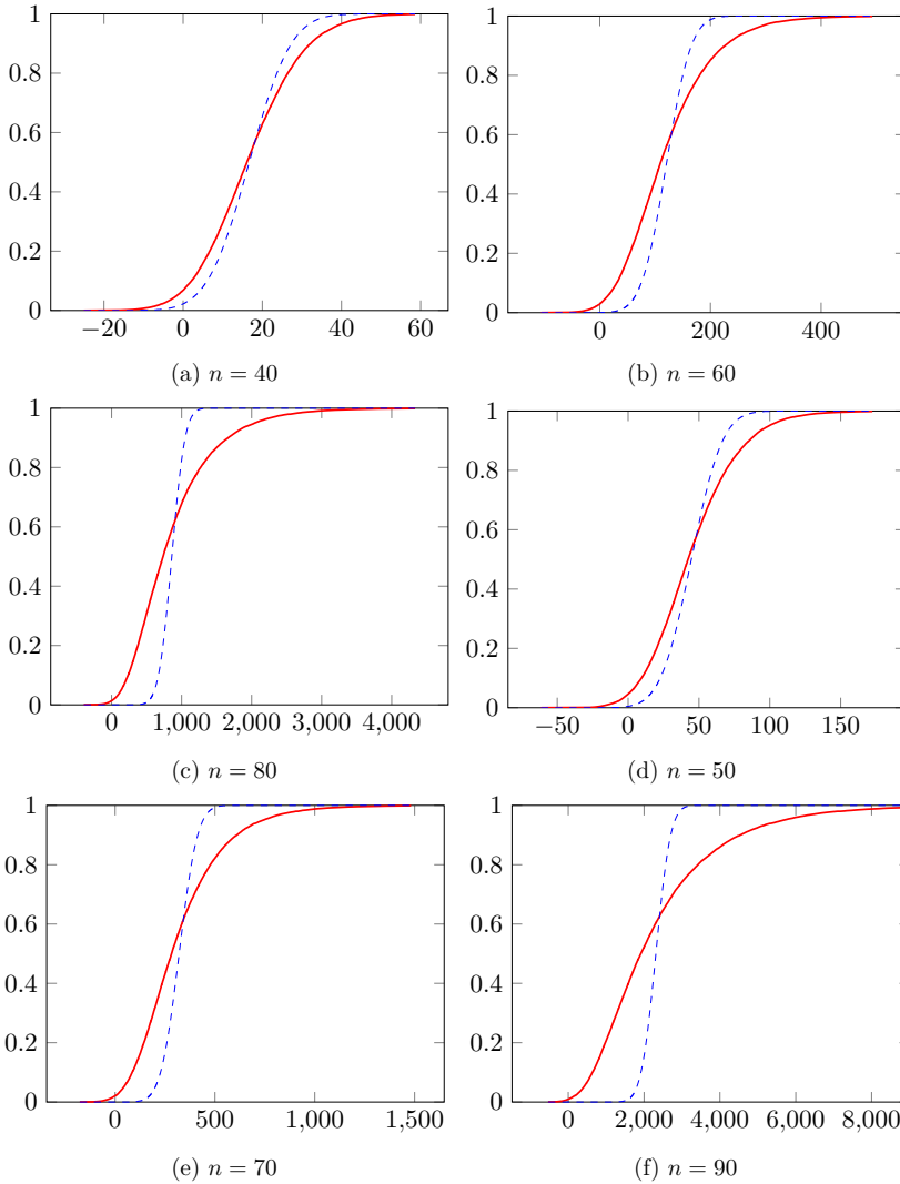
Figure 3.5: CDF of the score for Gaussian BDD targets in various dimensions n , with parameter \sigma = 0.7 \cdot \text{GH}(n)/\sqrt{n} , according to prediction from the Heuristic Analysis (dashed blue line), and experiments (red line). Each experimental curve has 2^{15} samples, which were obtained with code/bdd_scores.py and are listed in data/bdd_scores_nX.csv of the auxiliary files.
